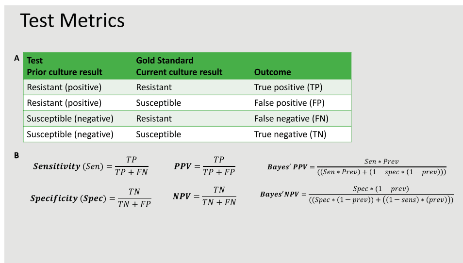
Figure 1. Test metric derivation (A) and formulas (B) used to calculate sensitivity (Sen), specificity (Spec), traditional positive predictive value (PPV), negative predictive value (NPV), and Bayes’ PPV and NPV. Prev indicates prevalence.
