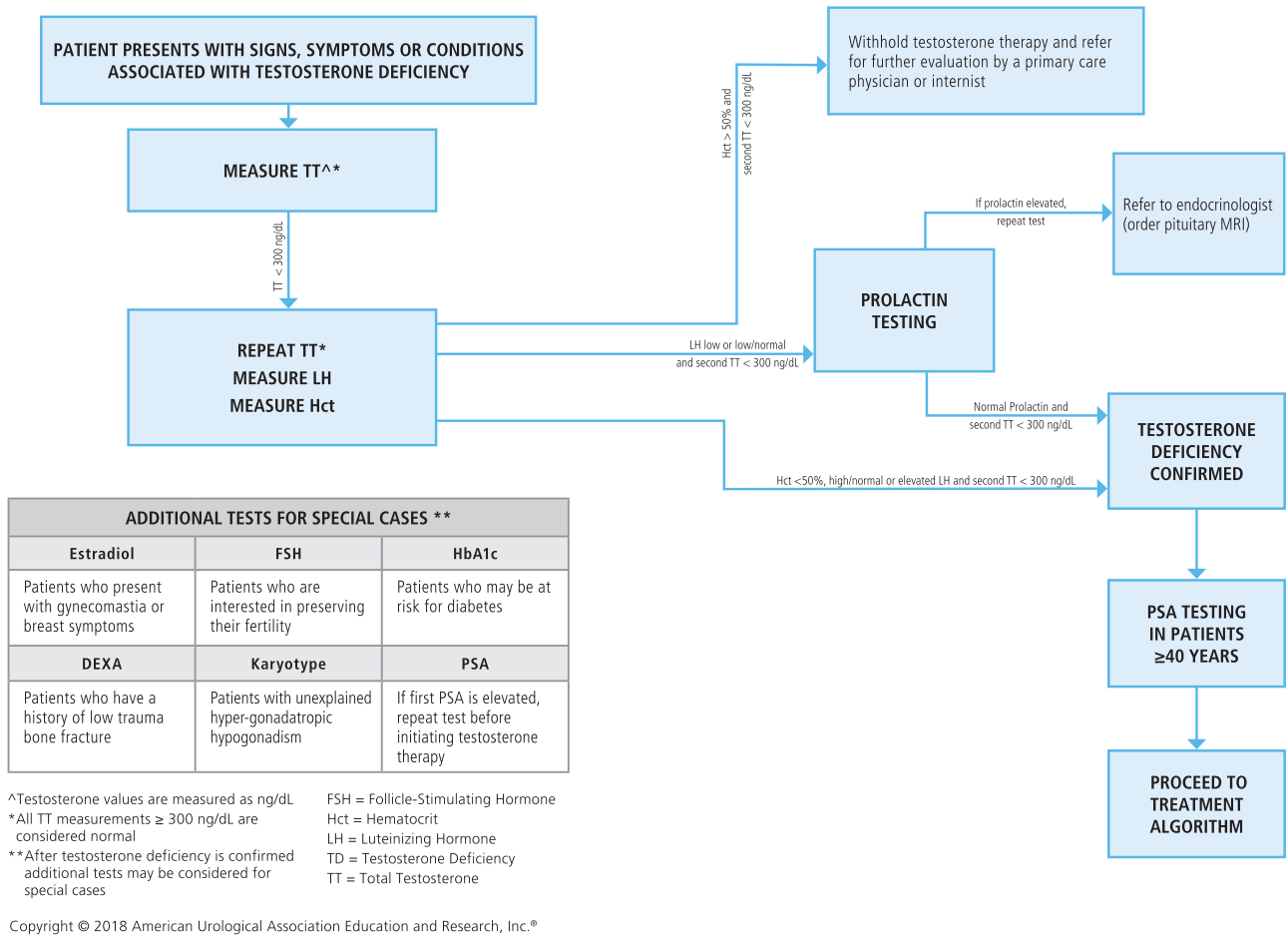
Figure 1. Diagnostic algorithm
